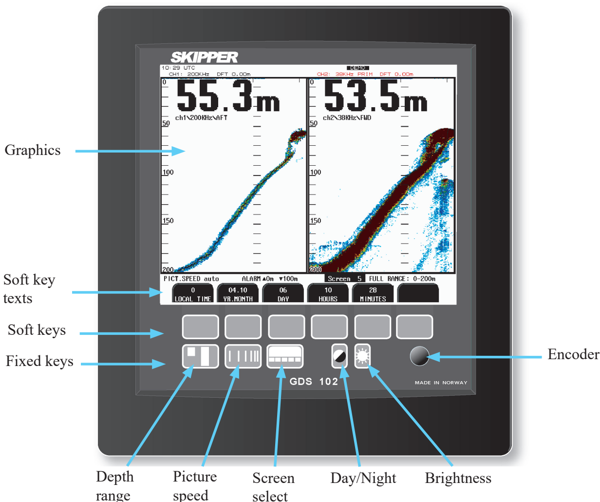
Fig. 1.1 Operator Unit Panel Layout
