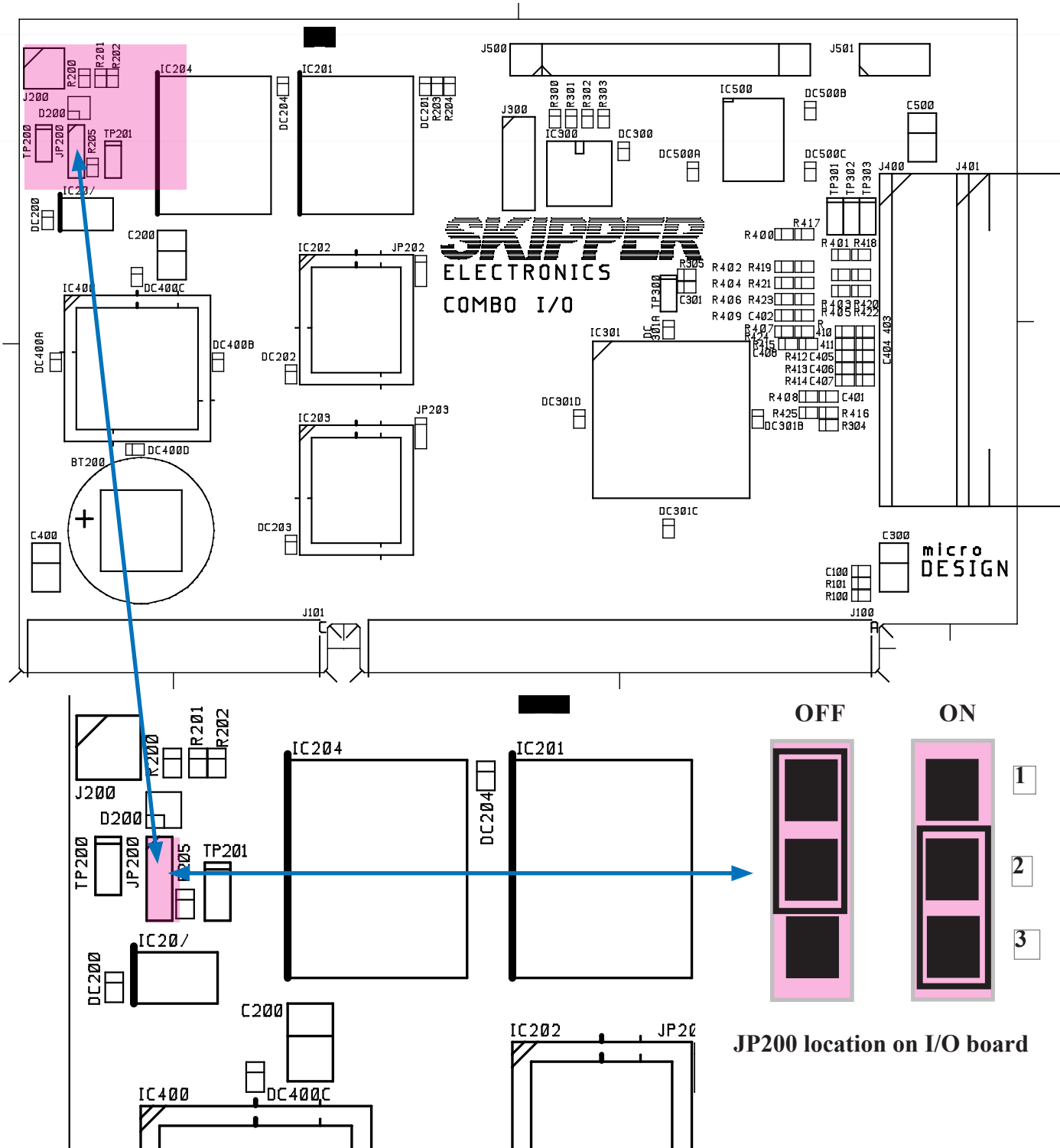
Fig. 3.7. Back-up battery jumper JP200, on I/O board.
